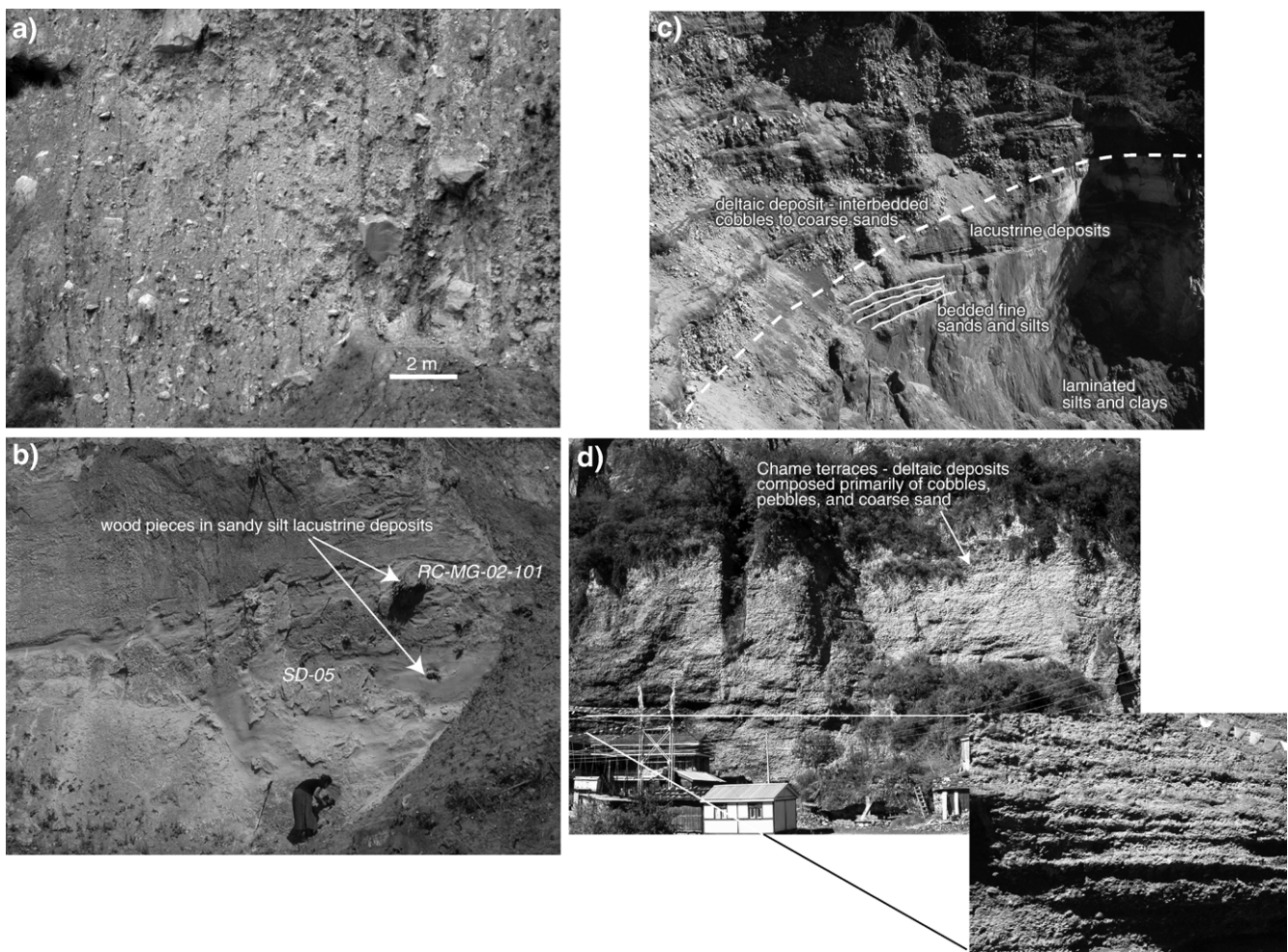
Figure 4. (a) Landslide dam diamicton. (b) Nar Khola sandy silt lacustrine deposits. Collection site for ^{14}\text{C} samples RC-MG-02-101, RC-MG-02-102, and RSA-97-2 and sediment sample SD-05. (c) Ghatte Khola contact between deltaic and lacustrine deposits. (d) The Chame terraces deltaic deposits, full vertical view and close-up.
